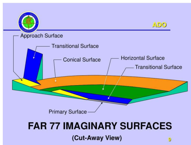
Figure 6-8: FAR Part 77 Imaginary Surfaces
