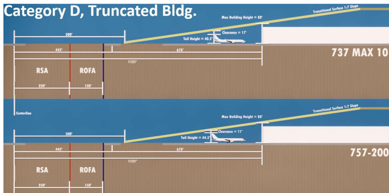
Figure 6-12: Category D Instrument Approach, Truncated Building with Aircraft Parking Position Setback
