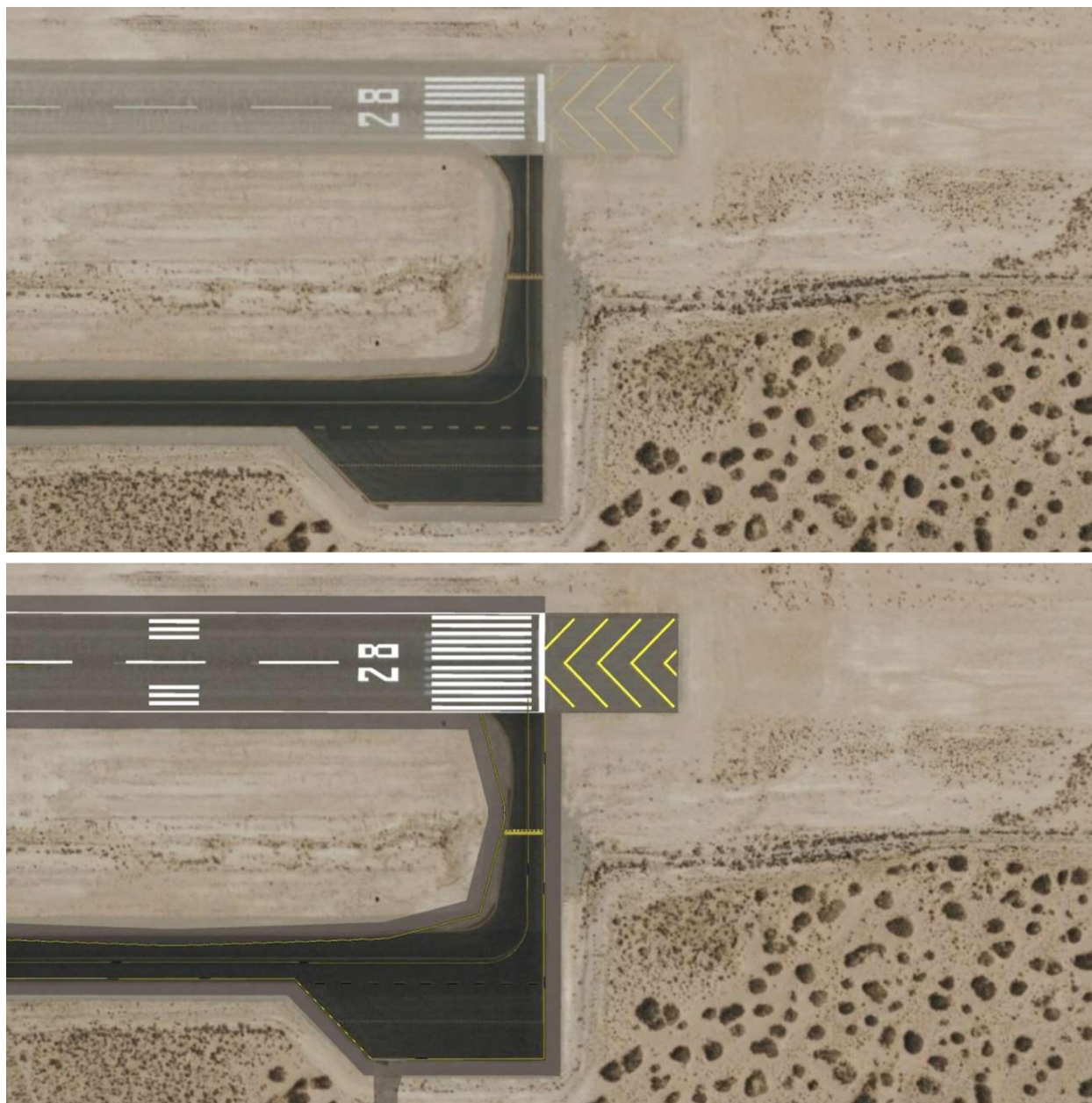
Figure 6-5: Runway 28 End Taxiway Fillets – Existing (Top) vs. TDG-4 (Bottom)
