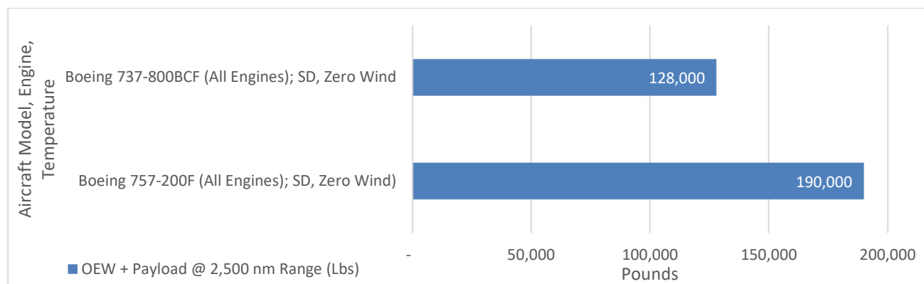
Figure 5-12: Comparison of Payload/Range Operating Empty Weight + Payload (Pounds) at 2,500 Nautical Miles on Standard Day with Zero Wind – Boeing 737-800BCF vs Boeing 757-200F
