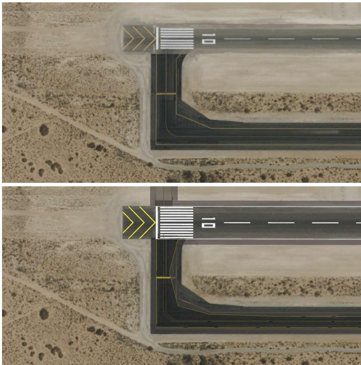
Figure 6-6: Runway 10 End Taxiway Fillets – Existing (Top) vs. TDG-4 (Bottom)
