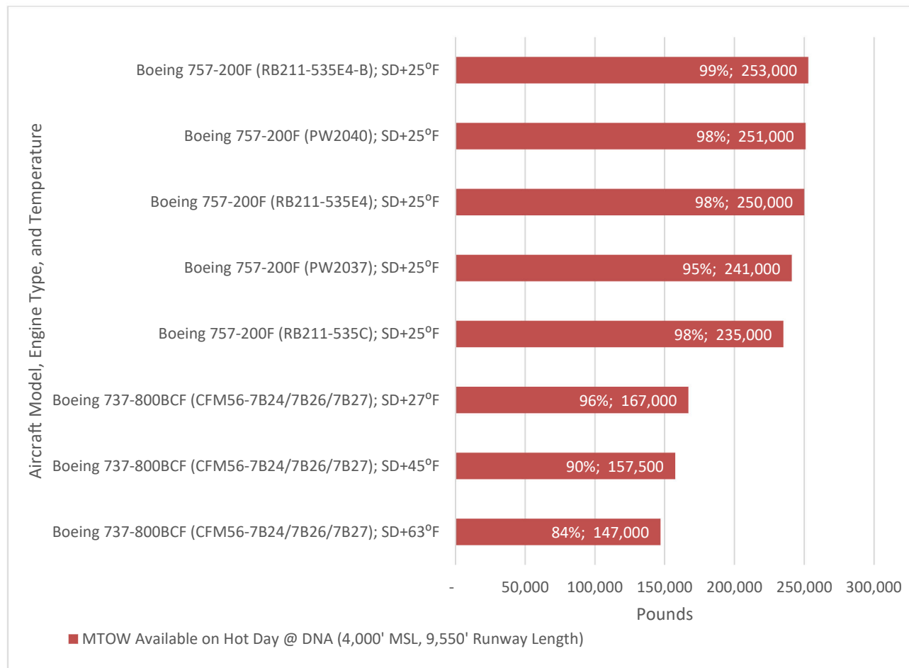
Figure 5-11: Comparison of Percent of MTOW Available on Hot Day at DNA (4,000' MSL; 9,550' Runway Length) – Boeing 737-800BCF vs Boeing 757-200F
