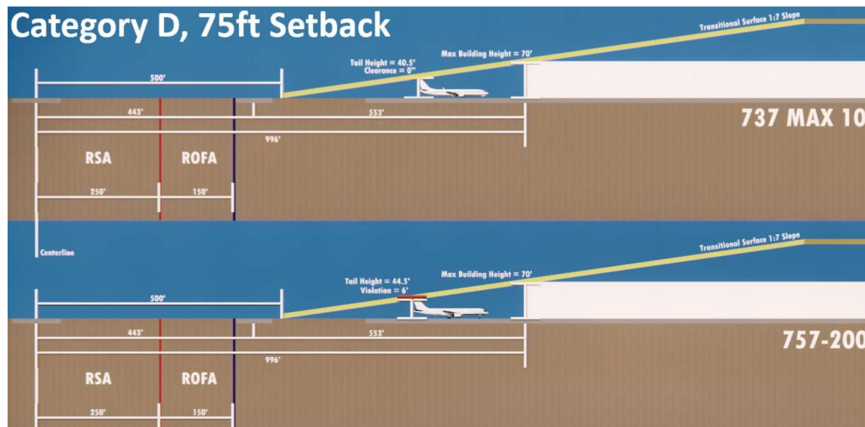
Figure 6-11: Category D Instrument Approach, 75-Foot Aircraft Parking Position Setback
