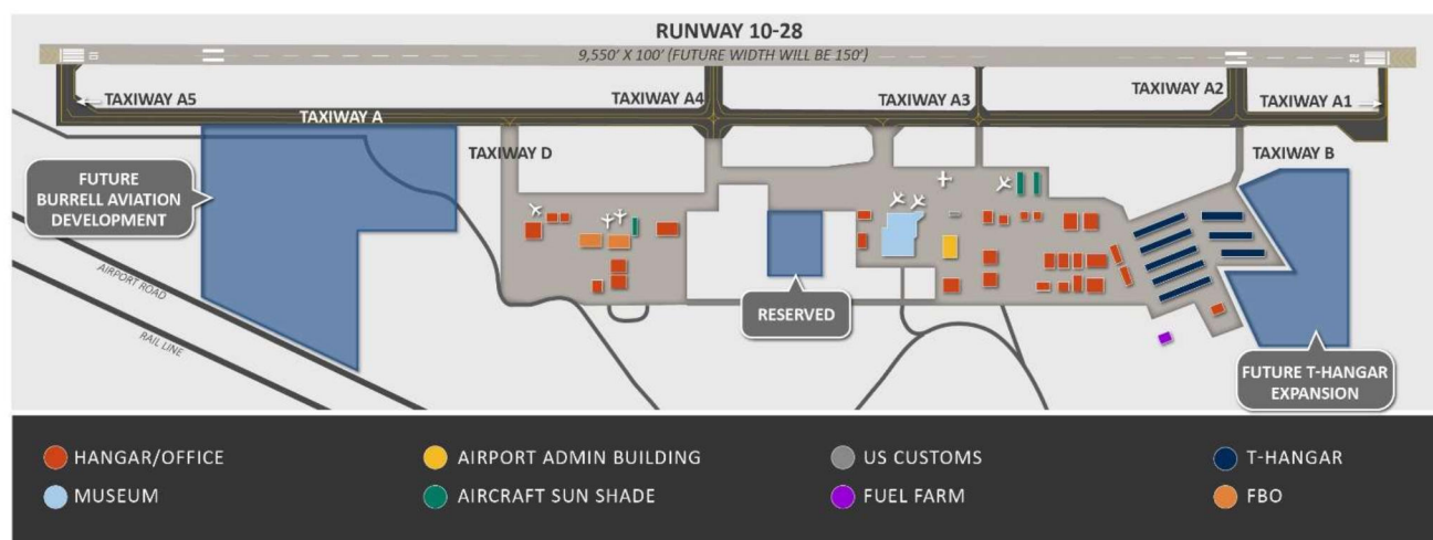
Figure 3-5: Apron Areas and Taxilanes
