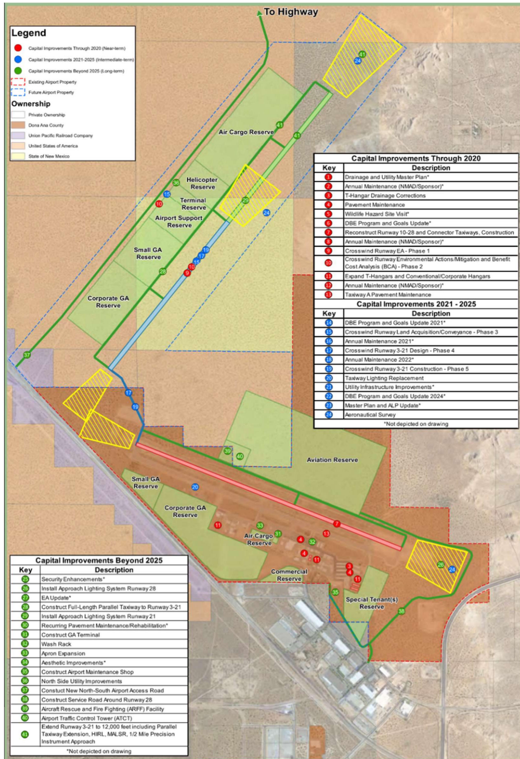
Figure 3-6: DNA Multi Modal Master Plan 2017 Overview
