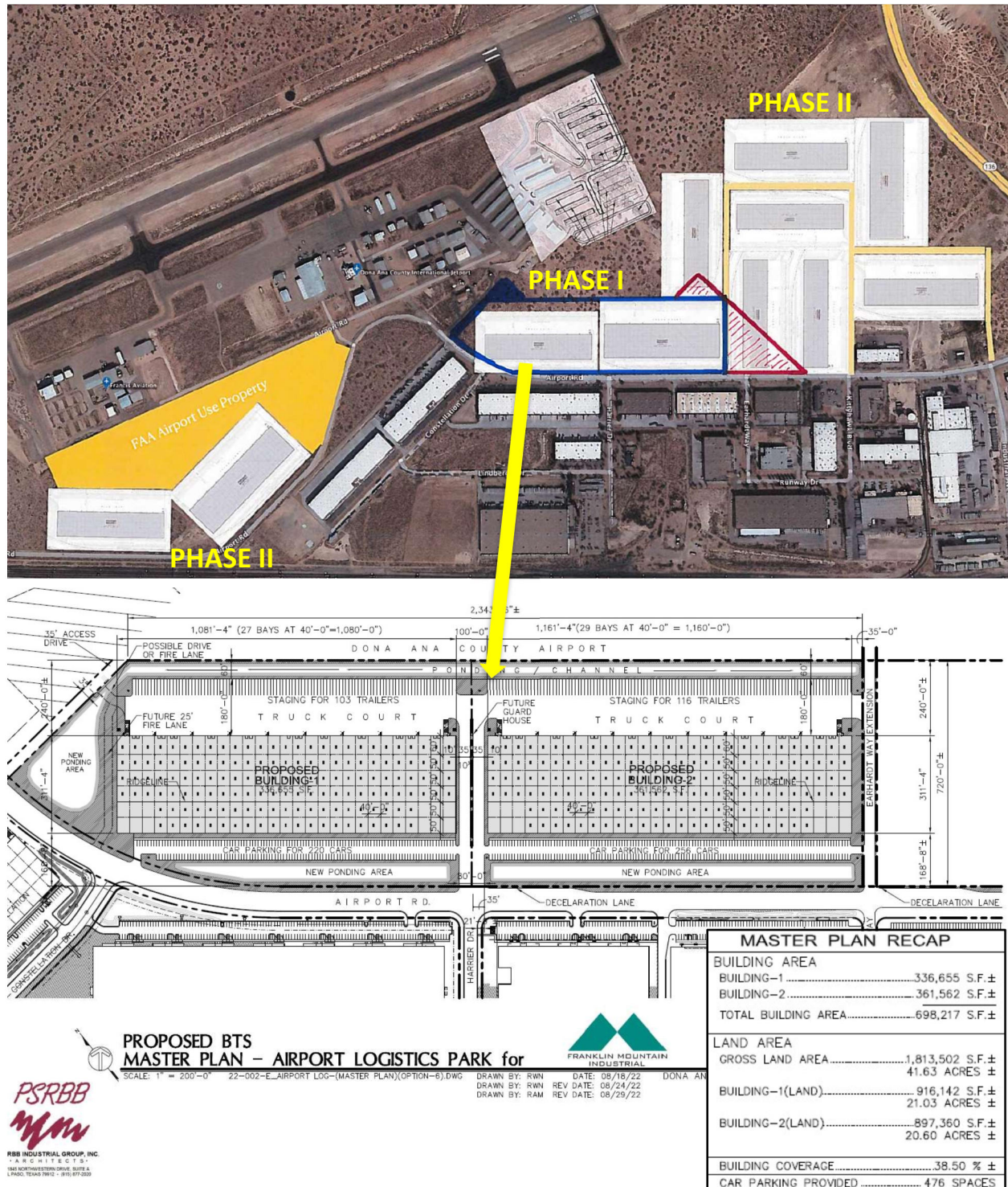
Figure 3-8: Future Non-Aeronautical Development Plan
