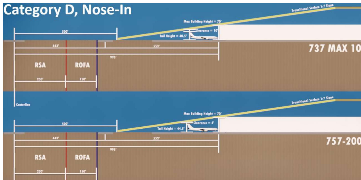
Figure 6-10: Category D Instrument Approach; Nose-In Configuration
