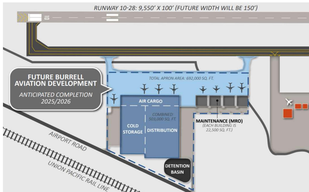
Figure 3-7: Future Cargo and Warehouse Facilities
