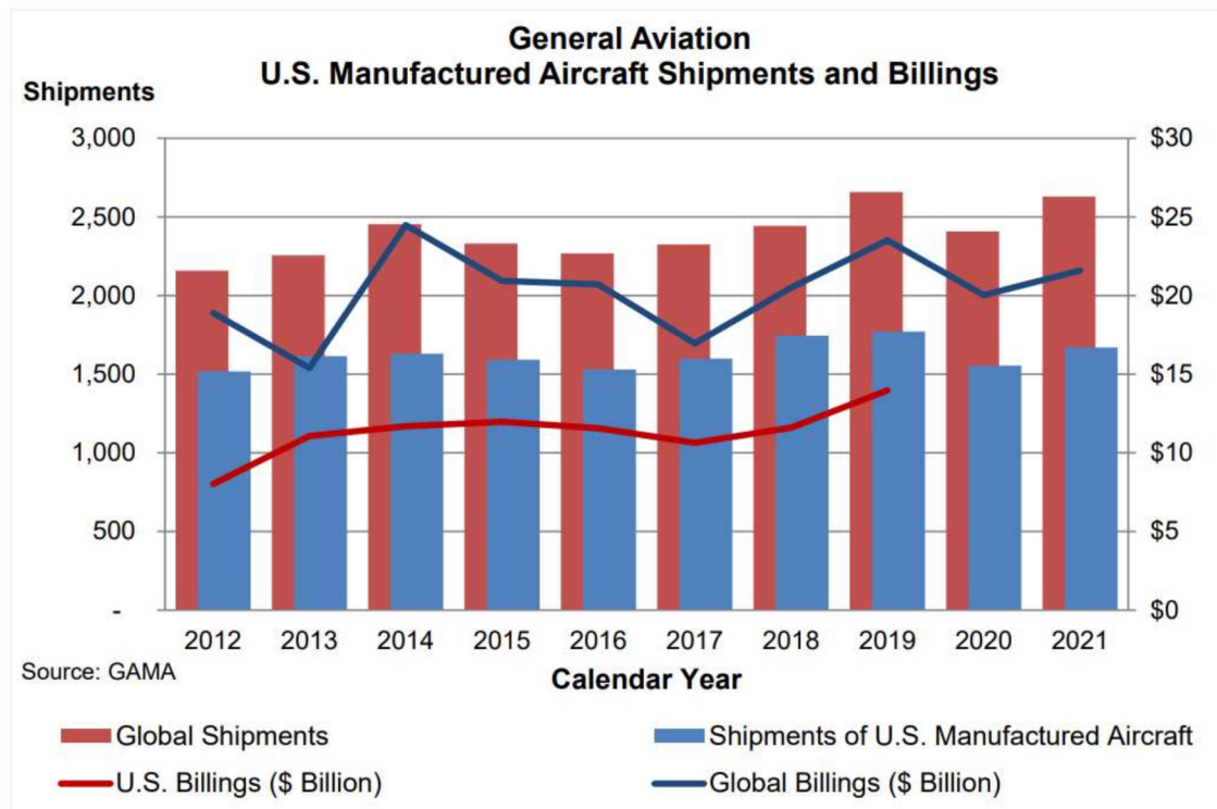
Figure E. Aircraft Shipments and Billings (Chart from FAA Aerospace Forecasts 2022-2042)
