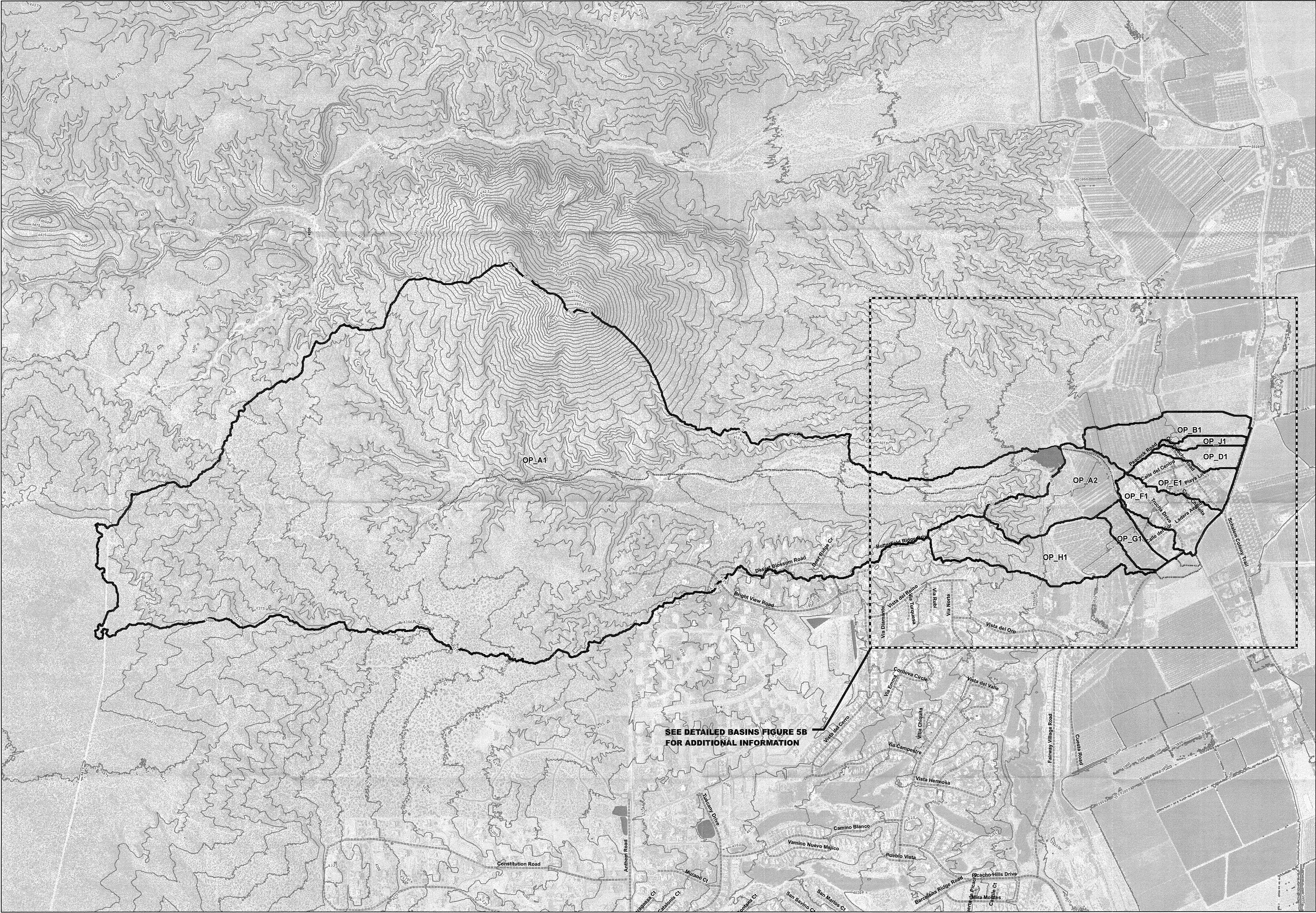
OLD PICACHO DRAINAGE MASTER PLAN BASIN MAP FIGURE 5A
