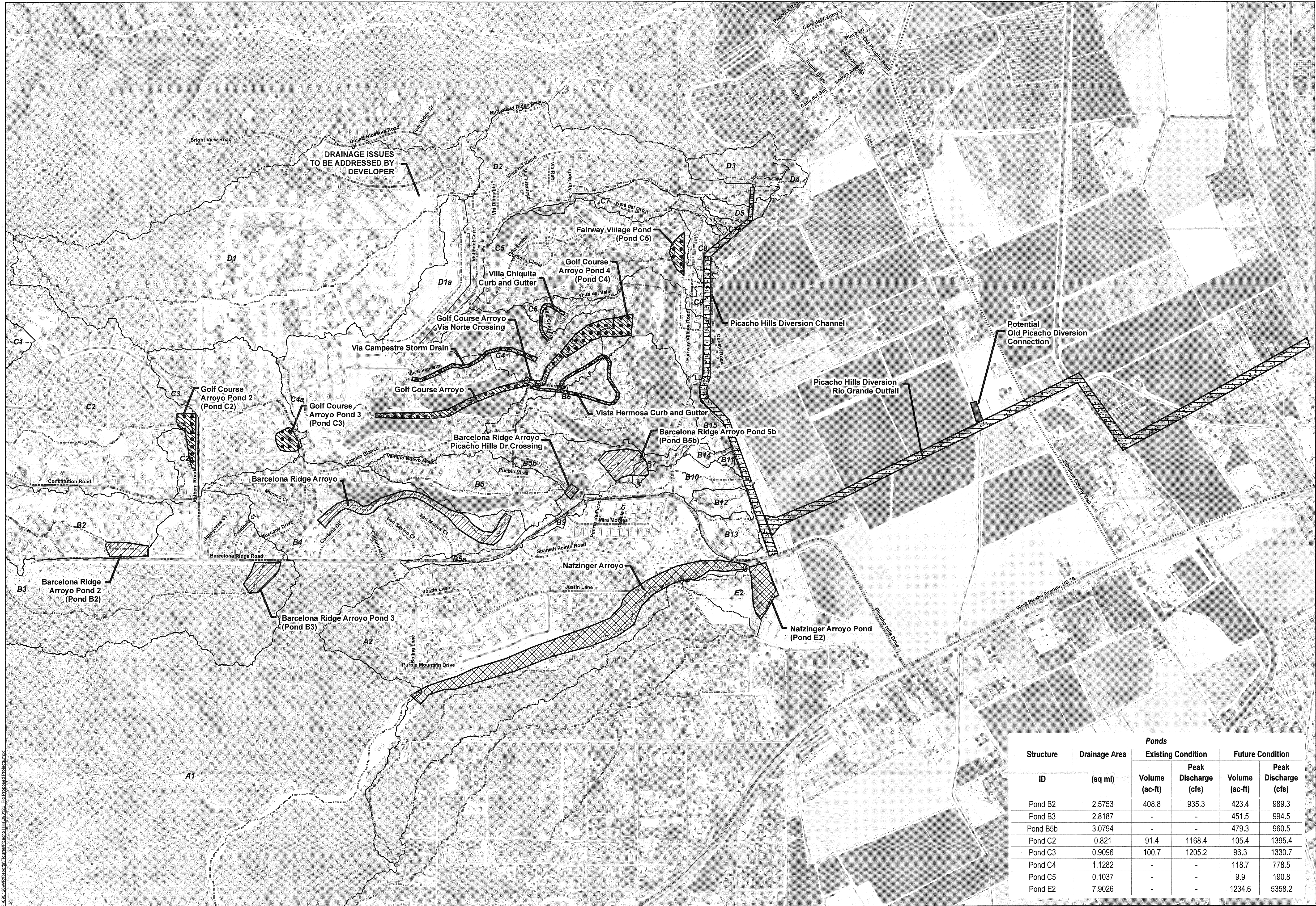
PICACHO HILLS DRAINAGE MASTER PLAN PROPOSED PROJECTS FIGURE 7
