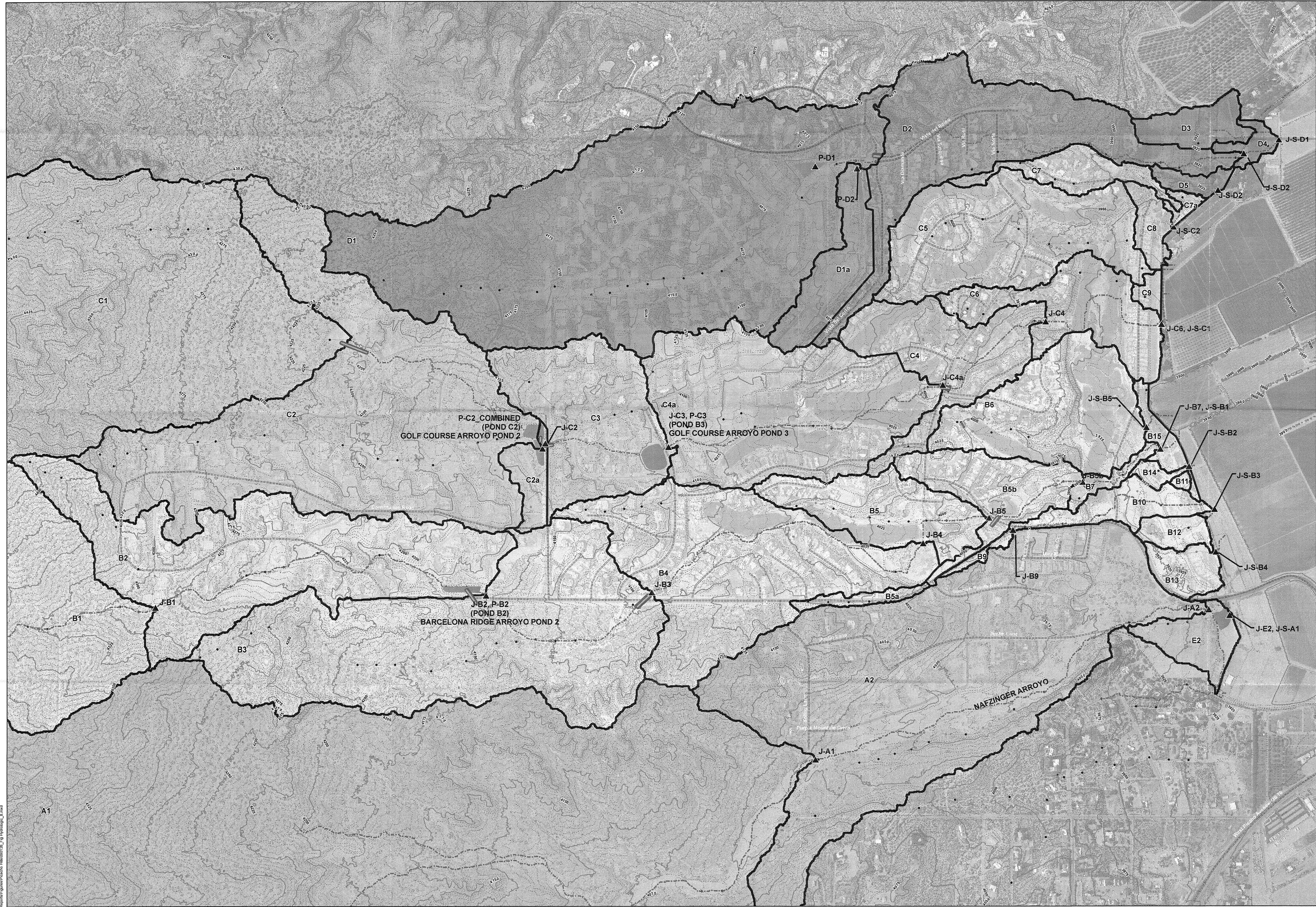
PICACHO HILLS DRAINAGE MASTER PLAN DETAILED BASIN MAP FIGURE 5B
