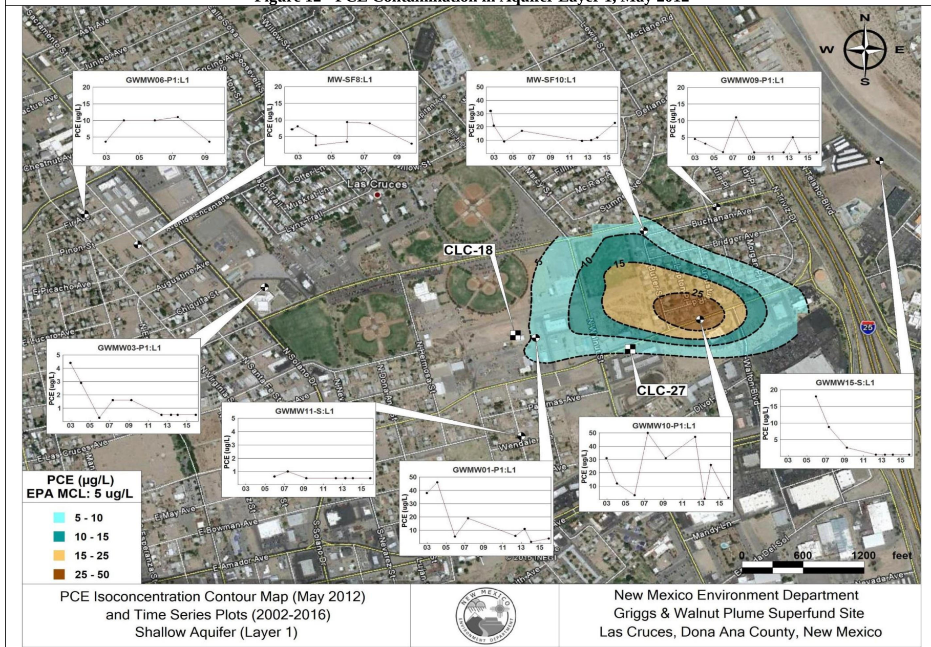
Figure 12 - PCE Contamination in Aquifer Layer 1, May 2012
