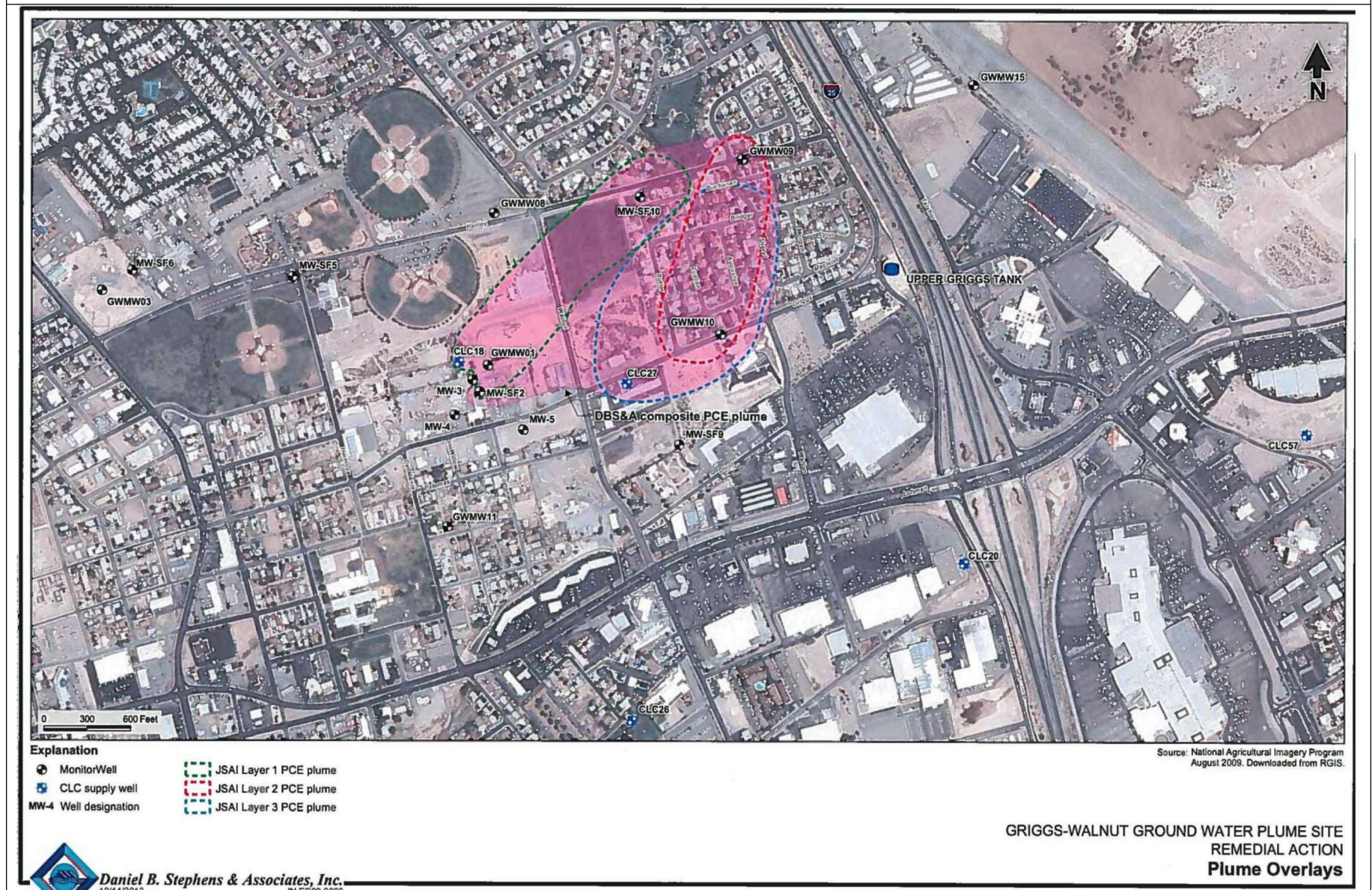
Figure 12 – Composite PCE Contaminant Plume Overlays, Aquifer Layers 1, 2, and 3, 2012 (DBS&A, 2013)
