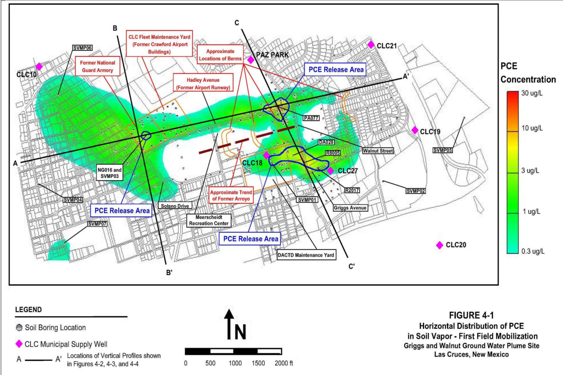
Figure 2 – PCE Release Areas
