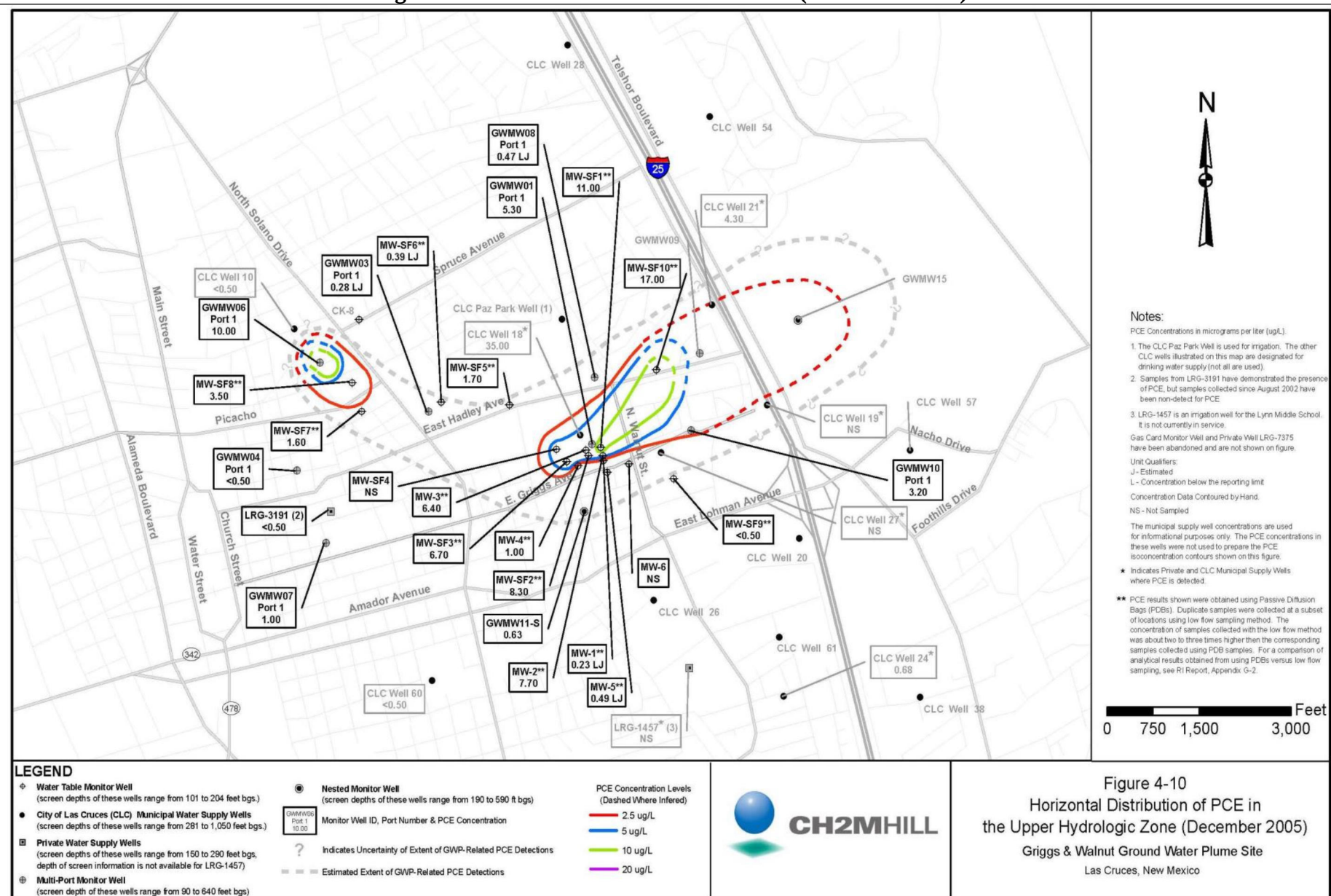
Figure 4 – PCE Groundwater Plume Area (December 2005)
