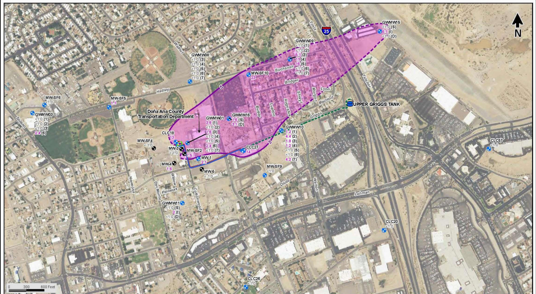
Figure 94 - PCE Contamination in Groundwater, 2015, (DBS&A, 2016)
