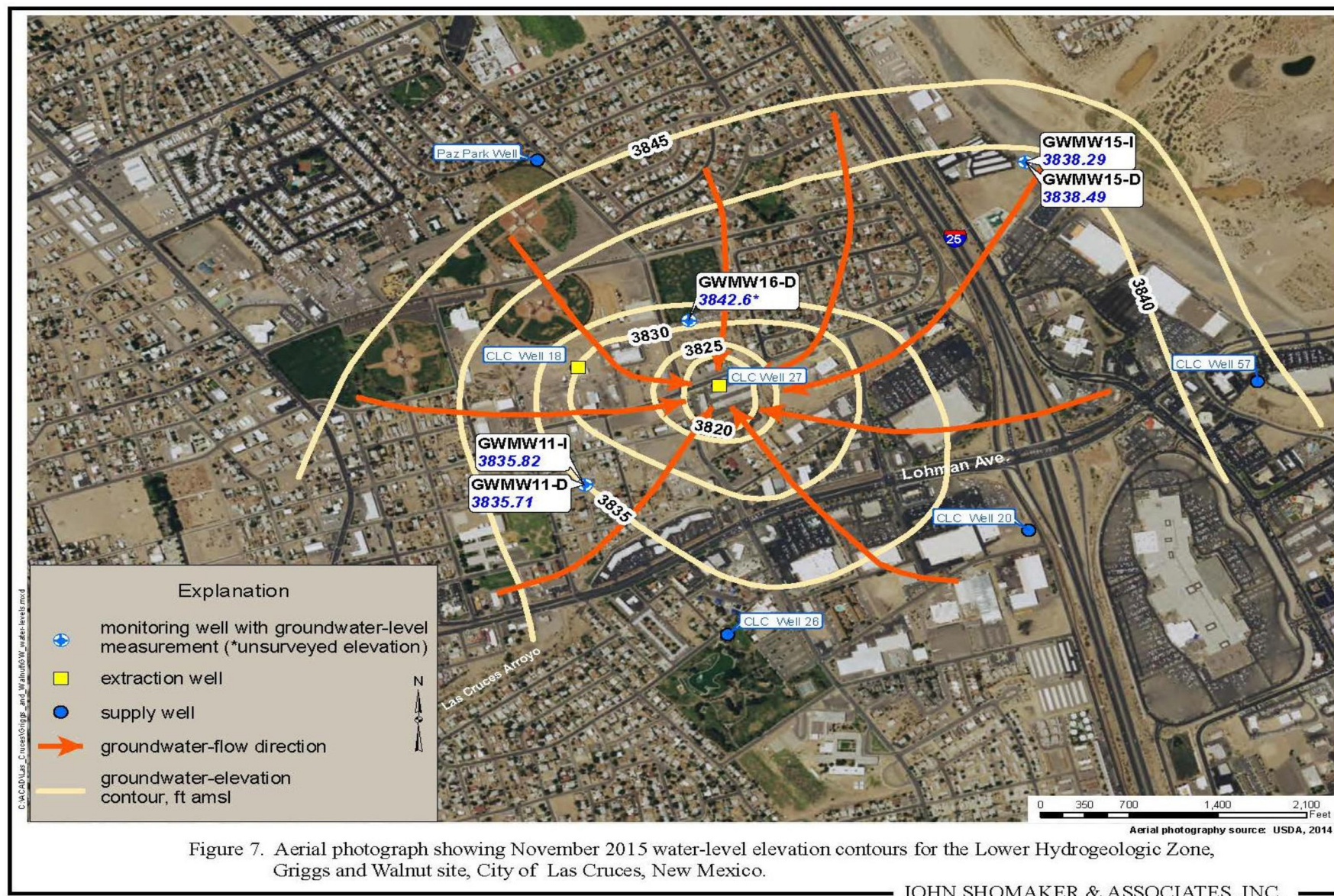
Figure 11 – Ground Water Elevation Contours for the Lower Hydrogeologic Zone November 2015 (JSAI, 2016)
