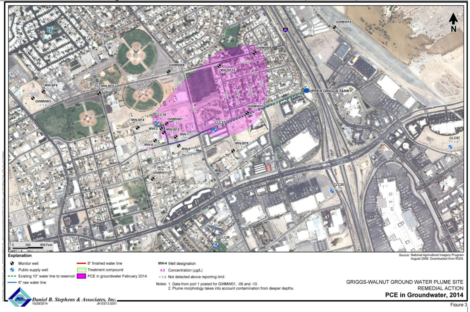
Figure 13 - PCE Contamination in Groundwater, 2014, (DBS&A, 2014)
