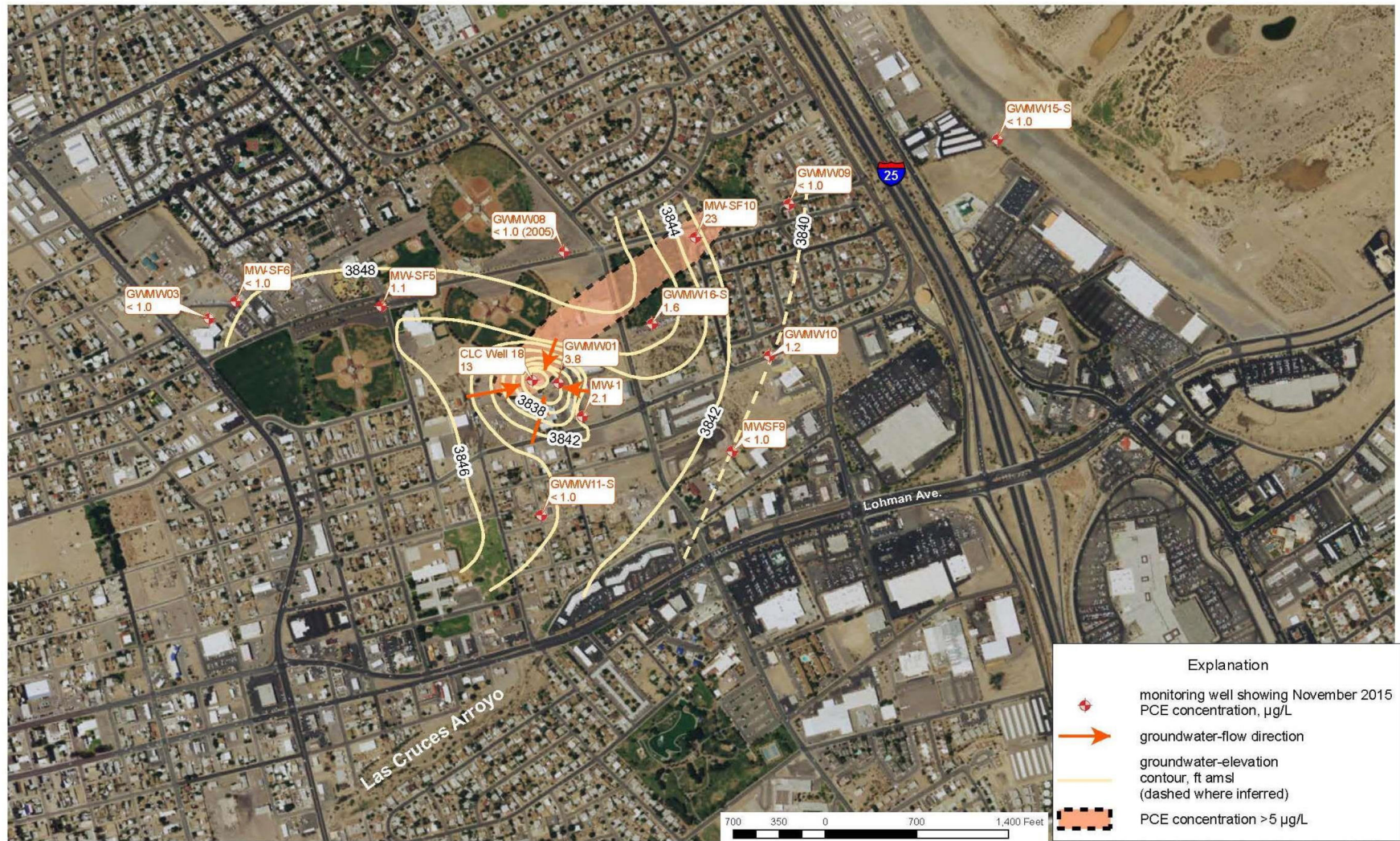
Figure 8 – Ground Water Elevation Contours for the Upper Hydrogeologic Zone and PCE Plume November 2015 (JSAI, 2016)
